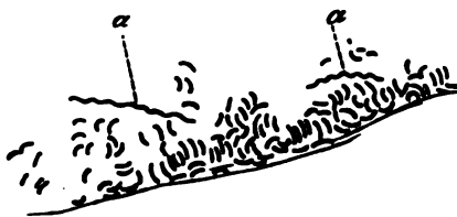
FIG. 85.—COVER-GLASS PREPARATION OF THE EDGE OF A DROP OF MEAT INFUSION, containing a pure cultivation of comma-bacilli, with (a) spirilliform threads, X 600 [after Koch].
